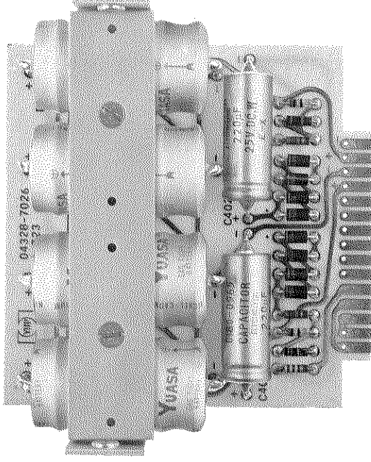
Figure 8-11. Model 4328A Ni-Cd Power Supply PC Board
