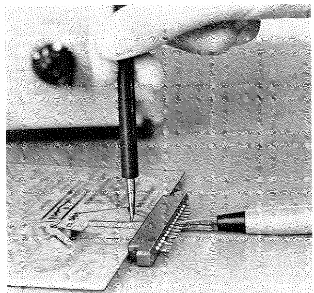
Figure 3-4. Probe Combination
