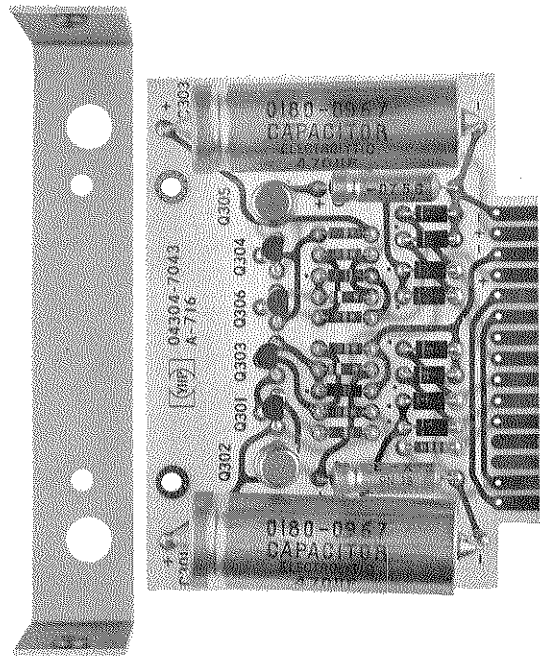
Figure 8-10. Model 4328A Power Supply PC Board
